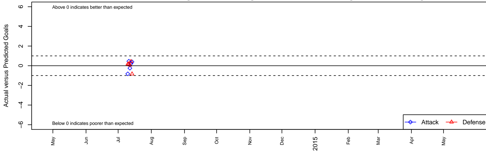
Sockers FC Chicago B98 Dots are actual minus expected GF (blue circles) and GA (red triangles). Blue line is smoothed change in attack strength. Red is smoothed change in defense strength.
